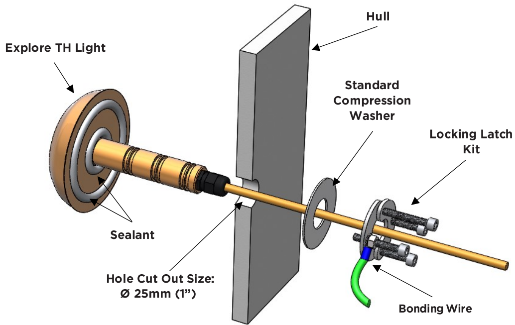
Exploded view of the assembly
